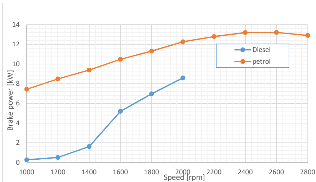
Figure 4.1: Graph of brake power against Speed
